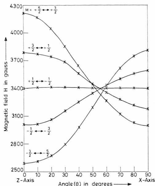
Fig. 1. Angular variation of the fine structure transitions of Mn 2+ for site I in the zx plane. The solid lines are smooth curves that connect data points from the same transition.
